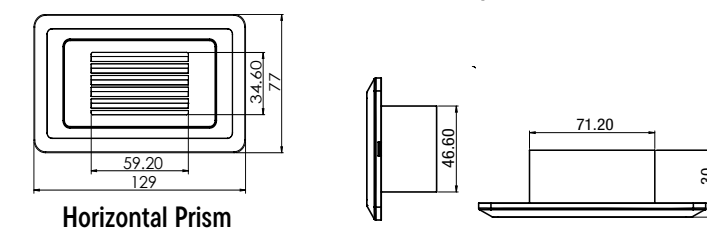
Prism and Louvre (Side & Top)
